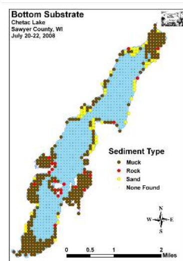
Figure 13 – Bottom Substrate From 2008 ERS Plant Survey
